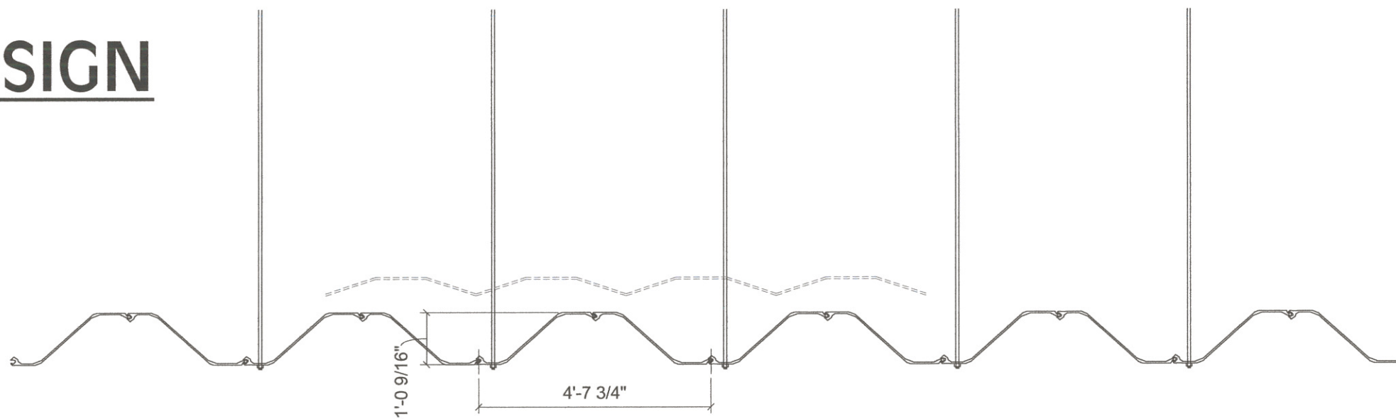
① PLAN VIEW 3/4" = 1'-0"
