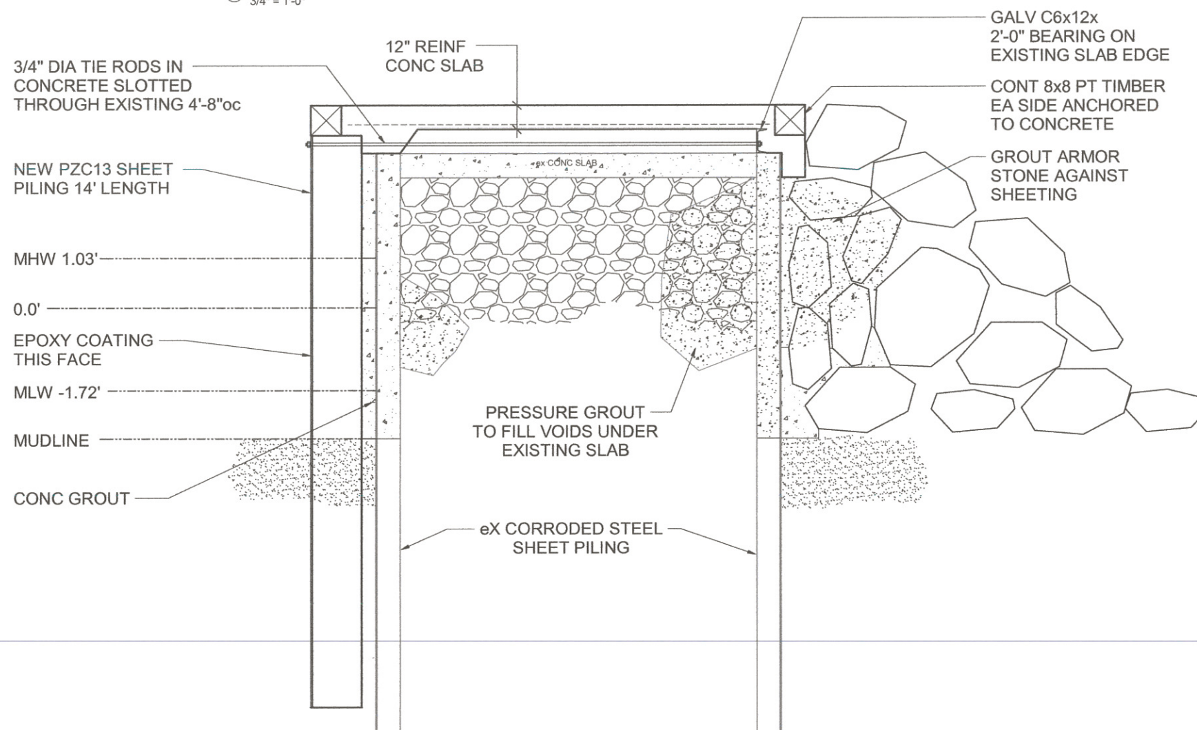
② SECTION VIEW 3/4" = 1'-0"
